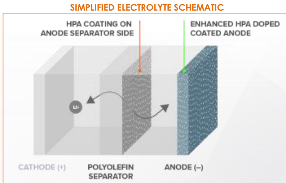
Figure: Lithium-ion battery showing the enhanced HPA doped coated anode and HPA particles on the polyolefin separator.
